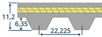
XH
