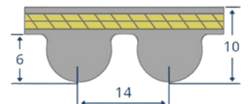
HTD 14M
