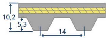
S14M
