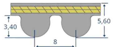
HTD 8M
