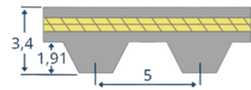
S5M
