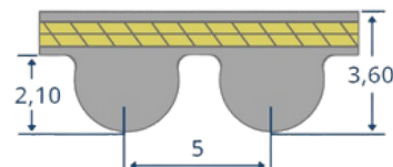
HTD 5M
