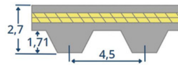
S4,5M
